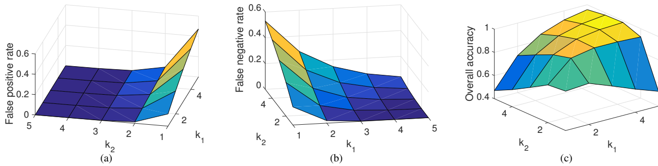
Fig. 10. Accuracy performance of advanced scheme.
