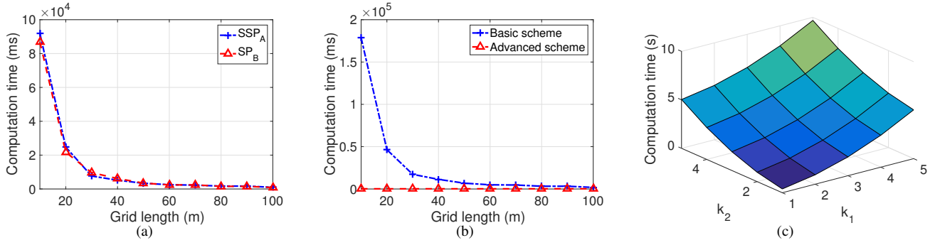
Fig. 7. Scheme performance on computation time.
